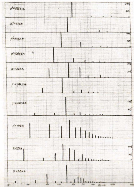
Tafel X Klangspektren Instrumenten-Körperschall offen - Mikrophon am Mundrohr (IV) Plate X Sound spectra Vibration of the instrument — open Pickup at the mouth tube (IV)
