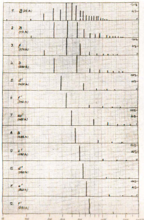
Plate I Sound spectra of the first 12 natural notes of the high B-flat horn
