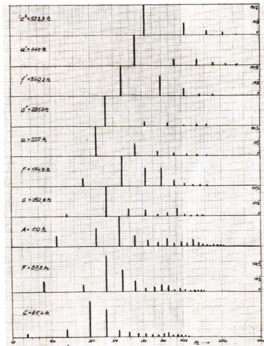
Tafel VIII Klangspektren Instrumenten-Körperschall offen - Mikrophon am Übergang Röhre Stürze (II) Plate VIII Sound spectra Vibration of the instrument — open Pickup at the joint between tube and bell (II)
