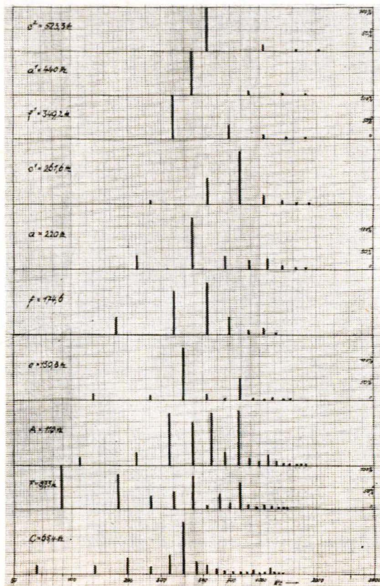
Tafel VII Klangspektren Instrumenten-Körperschall offen - Mikrophon am Kranz (I) Plate VII Sound spectra Vibration of the instrument — open Pickup at the rim (I)
