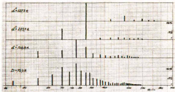
Plate III Spectra of the sounds d 2 , d 1 , d, D
