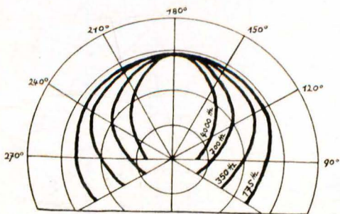
Abb. 20. Richtwirkungsdiagramm des Waldhorns (nach Stauder) für klingend f = 175 Hz " " f^1 = 350 Hz " " f^2 = 700 Hz " " c^5 = 4000 Hz Fig. 20. Polar diagram of the French horn (Stauder, loc. cit. par. 728, fig. 6) for f = 175 c/s, f^1 = 350 c/s f^2 = 700 c/s and c^5 = 4000 c/s
