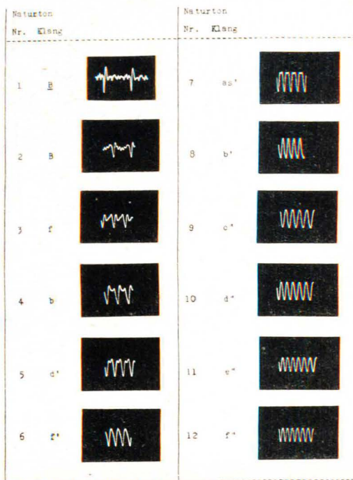
Plate II Oszillograms of the 1st 12 natural notes of the high B-flat horn
