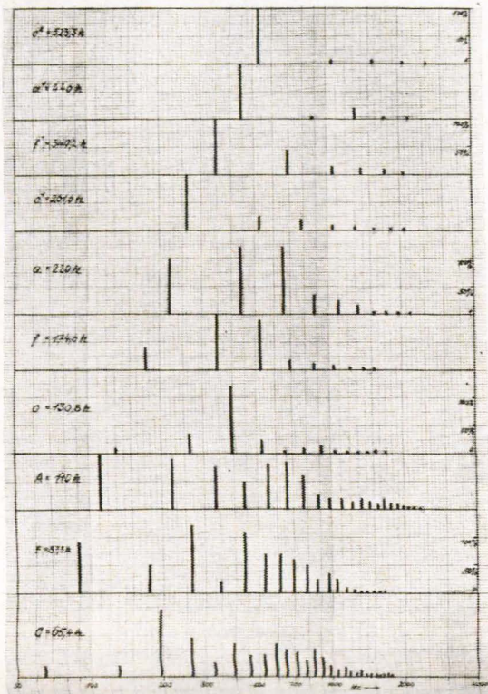
Tafel IX Klangspektren Instrumenten-Körperschall offen - Mikrophon am Rohr (III) Plate IX Sound spectra Vibration of the instrument — open Pickup on the tube (III)
